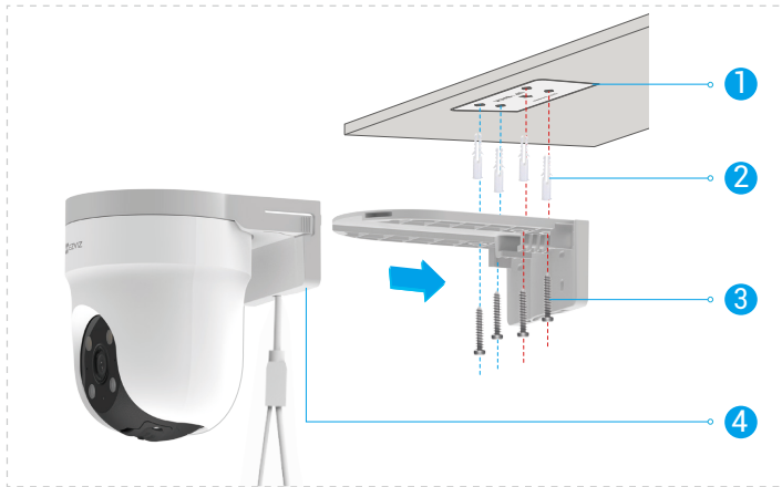
Fig. 1 Ceiling Mount
