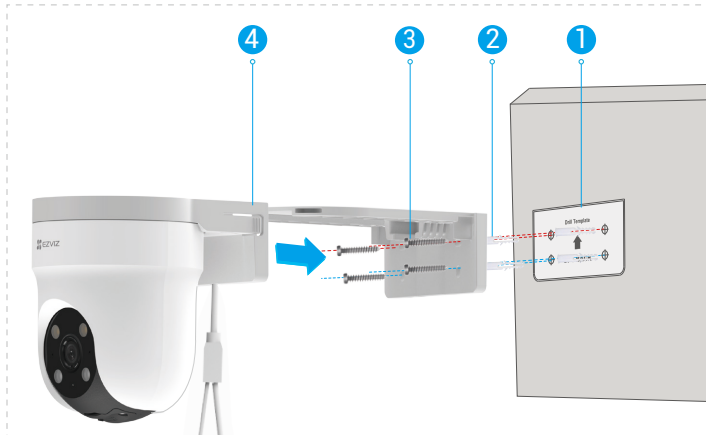
Fig. 2 Wall Mount
